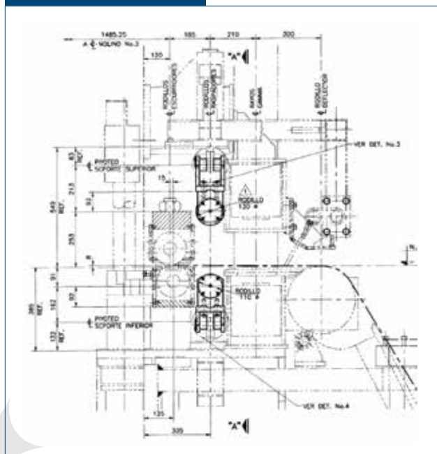
Roll configuration in the exit section.
