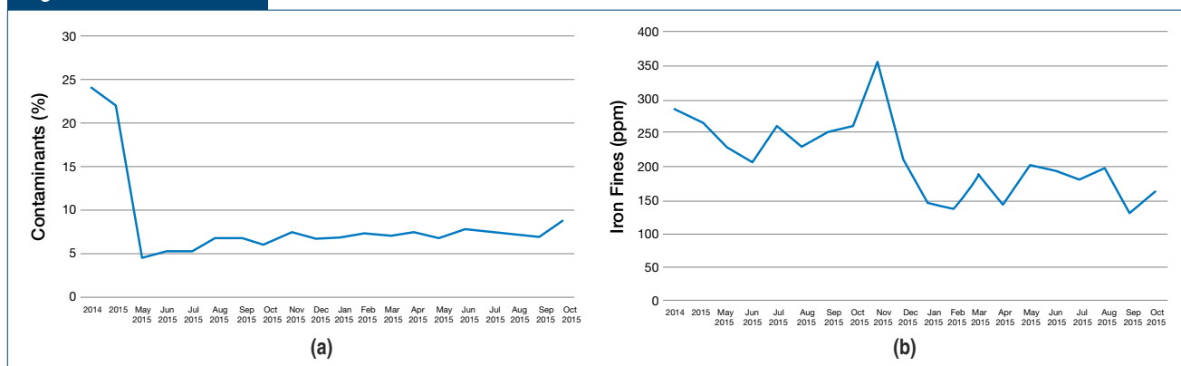
Oil solution: contaminants (tramps) (a) and iron fines (b).
