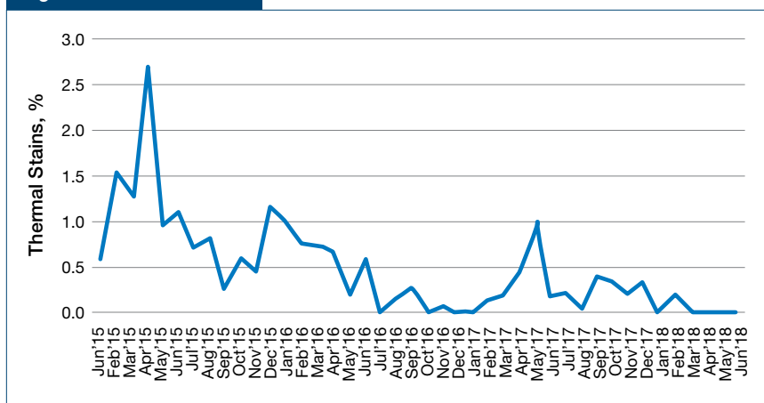
Thermal stains declassed material (2015–2018).
